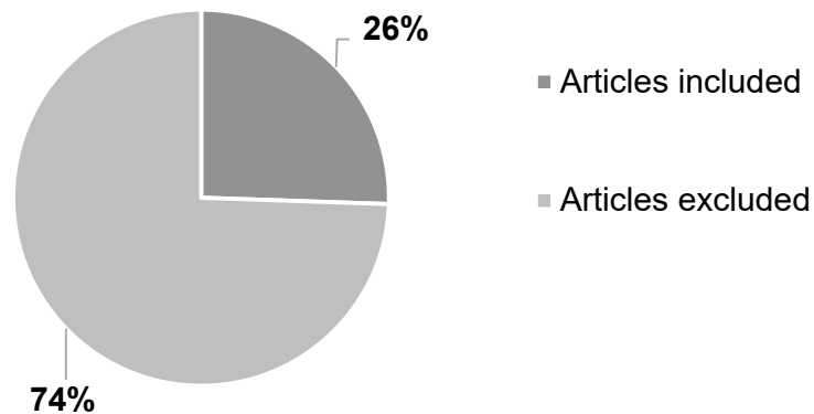
Figure 4. The number of articles included (dark grey) and excluded (light grey) in the systematic review, following the pre-defined inclusion and exclusion criteria.
