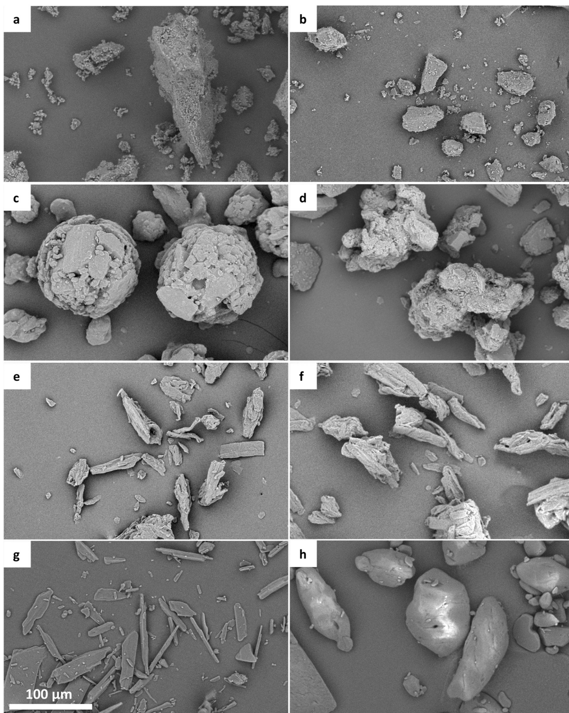
Fig. 1. Scanning electron micrographs of the six types of excipients and two API grades used in this study: a) anhydrous lactose, b) milled lactose monohydrate, c) spray dried lactose, d) granular lactose, e) MCC 101, f) MCC 102, g) paracetamol standard powder, h) paracetamol dense powder. The scale bar represents 100 \mu\text{m} .
