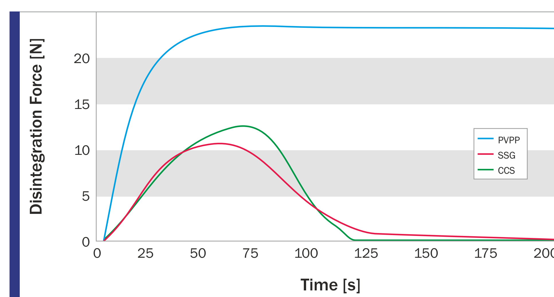
Fig. 1 Disintegration Force of Unconfined Tablets in Water
