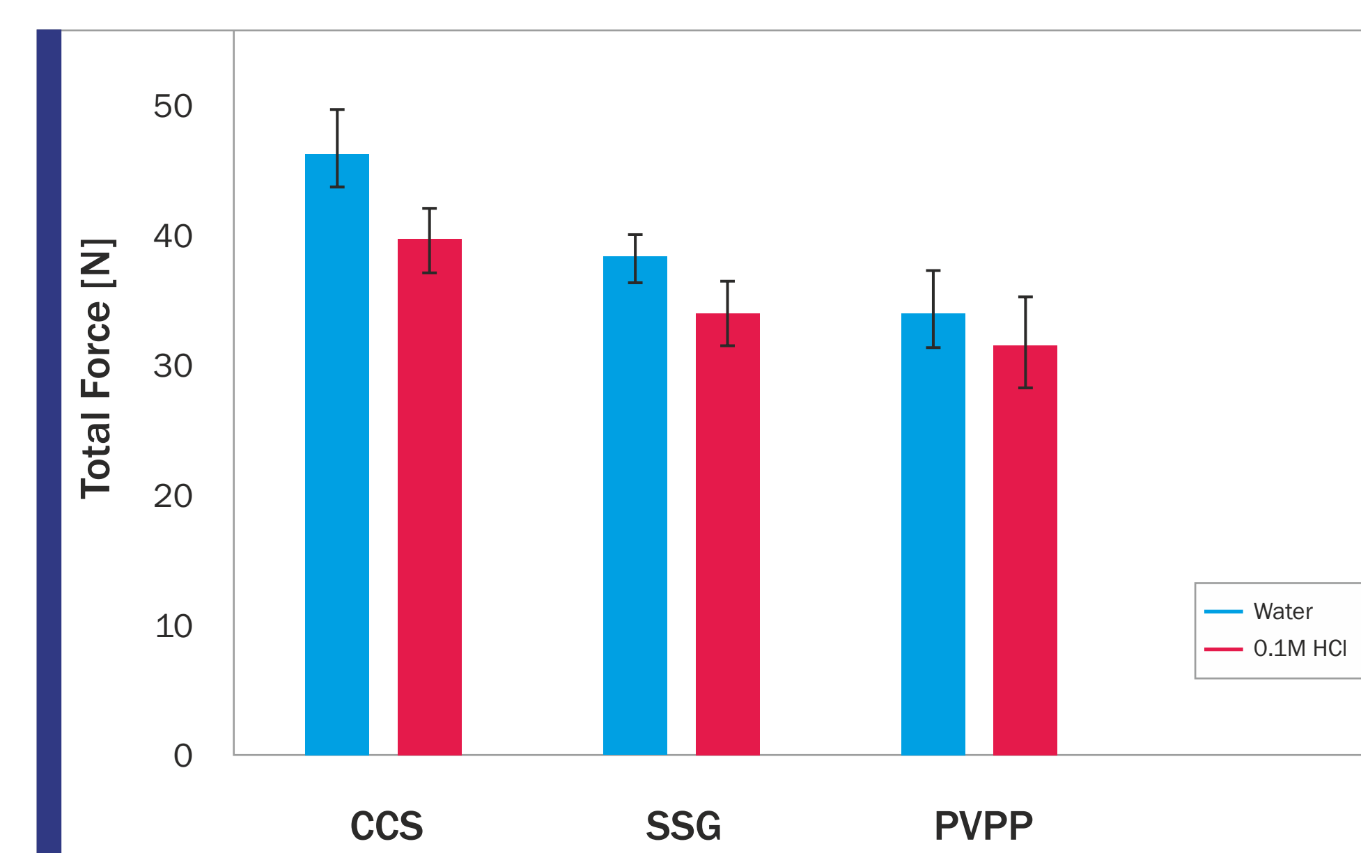
Fig. 3 Total Disintegration Force of Confined Tablets in Water and Hydrochloric Acid
