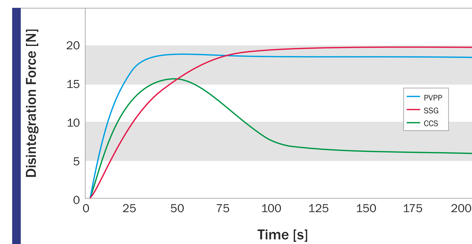
Fig. 2 Disintegration Force of Tablets in 0.1 M Hydrochloric Acid
