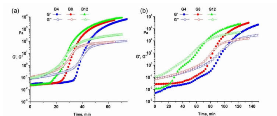
Figure 4. Comparative time sweep rheological test of (a) CD-PEG and (b) CDLA-PEG hydrogels syntheses.
