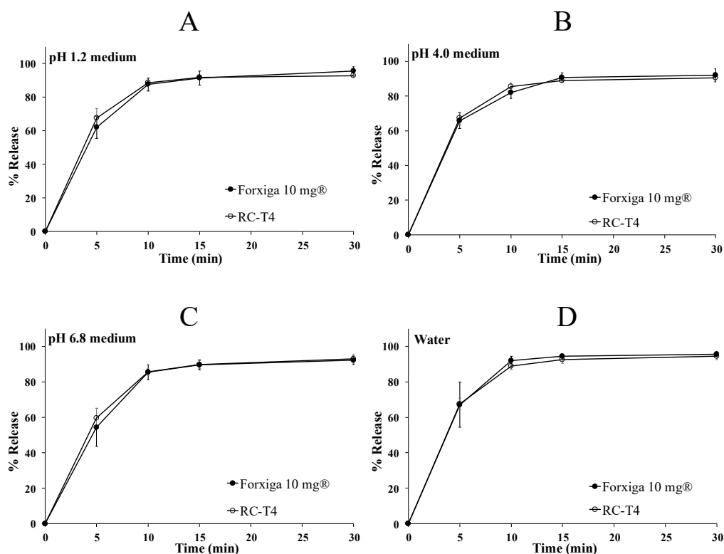
Figure 3. Dapagliflozin (DAP) dissolution profiles from Forxiga ® 10 mg and RC-T4 in pH 1.2 (A), pH 4.0 (B), pH 6.8 (C), and distilled water (D). The experiment was conducted in USP Apparatus 1 at 50 rpm and in dissolution media at 37.0 °C. Each value represents the mean \pm standard deviation ( n = 6 ).
