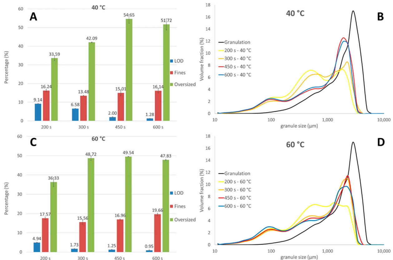
Figure 6. The fraction in fines and oversized granules and the corresponding overall moisture content after different drying times for granules collected after the conditioning unit at 40 (A) and 60 °C (C). Granules size distributions to visualize the effect of drying time at 40 (B) and 60 °C (D).
