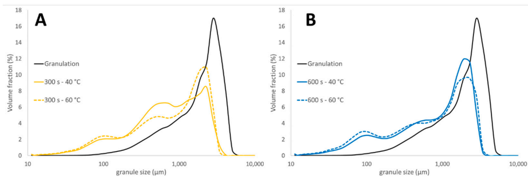
Figure 8. Granule size distribution to study the effect of drying air temperature on granule size after 300 (A) and 600 s (B) of drying.
