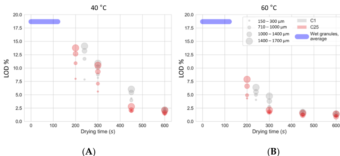
Figure 5. Residual moisture content (LOD values) of the granules produced on C1 and C25 in function of drying time at 40 °C (A) and 60 °C (B) for different size fractions (smaller size fractions are represented by smaller dots, whereas larger size fractions are represented by larger dots). The average moisture content of granules entering the drying cells during the filling phase was depicted by the blue bar.
