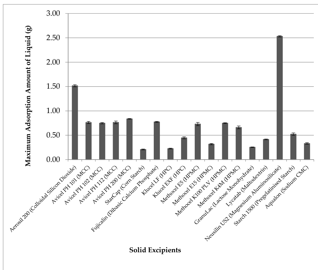
Figure 1. The maximum adsorption amount of liquid tocotrienol-rich fraction (TRF) on 1 g of different solid excipients (mean \pm SD, n = 3).
