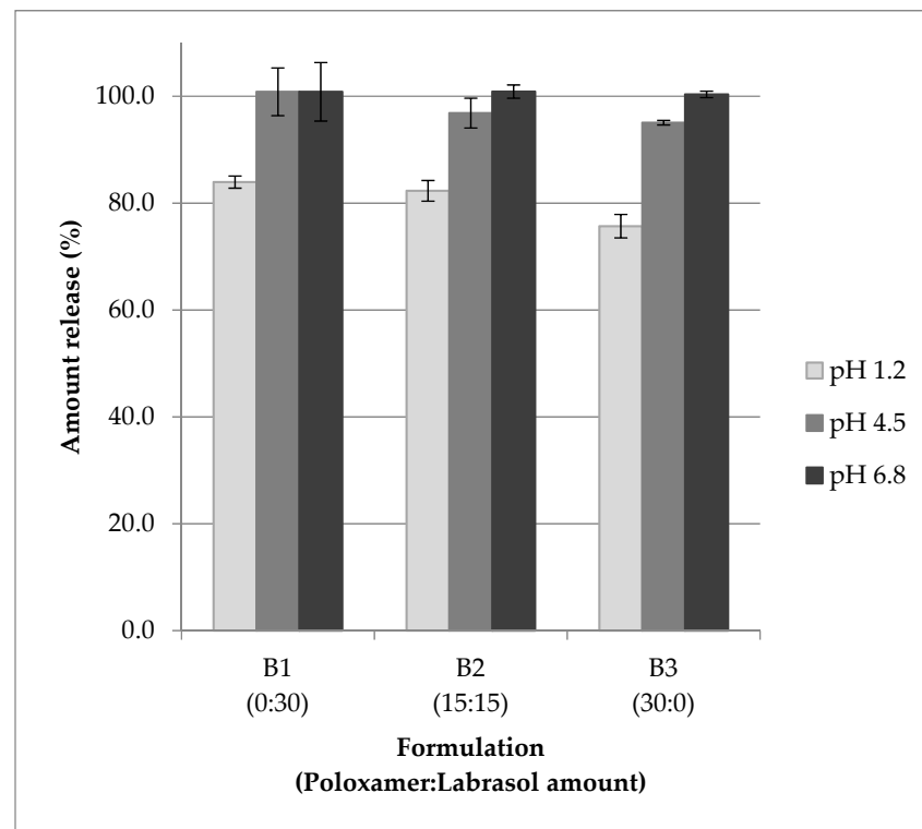
Figure 2. Amount of mixed tocotrienols release from s-SEDDS containing 70% TRF and 30% mixed surfactants in different pH (mean \pm SD, n = 3).
