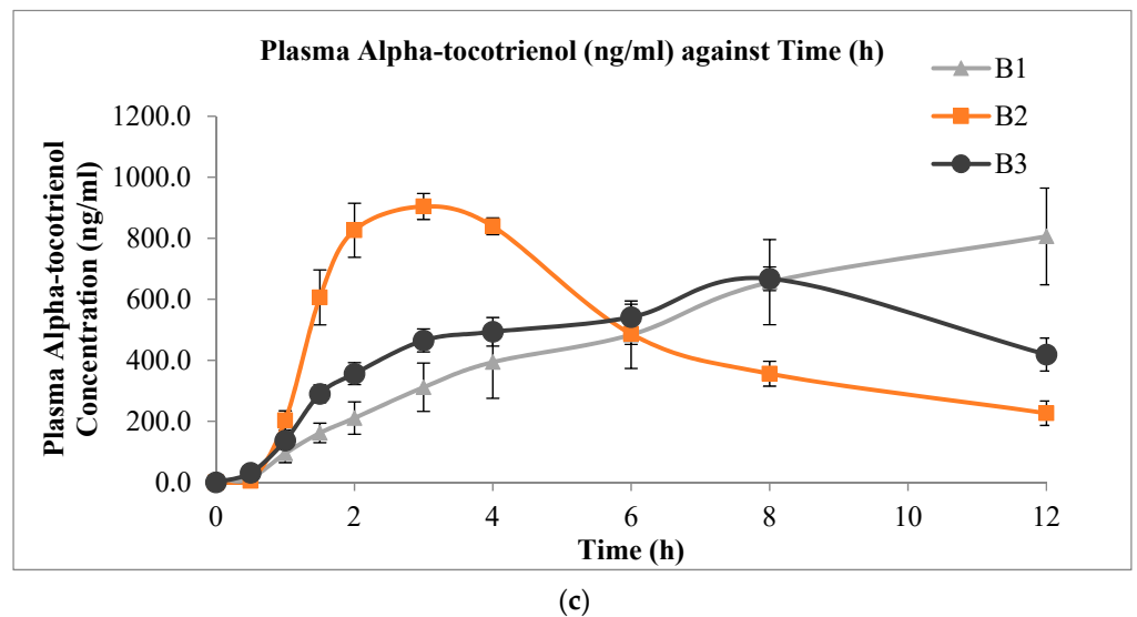
Figure 3. Mean plasma concentration versus time profiles (mean \pm SEM, n = 6 ) of (a) delta-tocotrienol; (b) gamma-tocotrienol; and (c) alpha-tocotrienol after oral administration of 20 mg/kg mixed tocotrienols in s-SEDDS containing 70% TRF and 30% surfactant(s).
