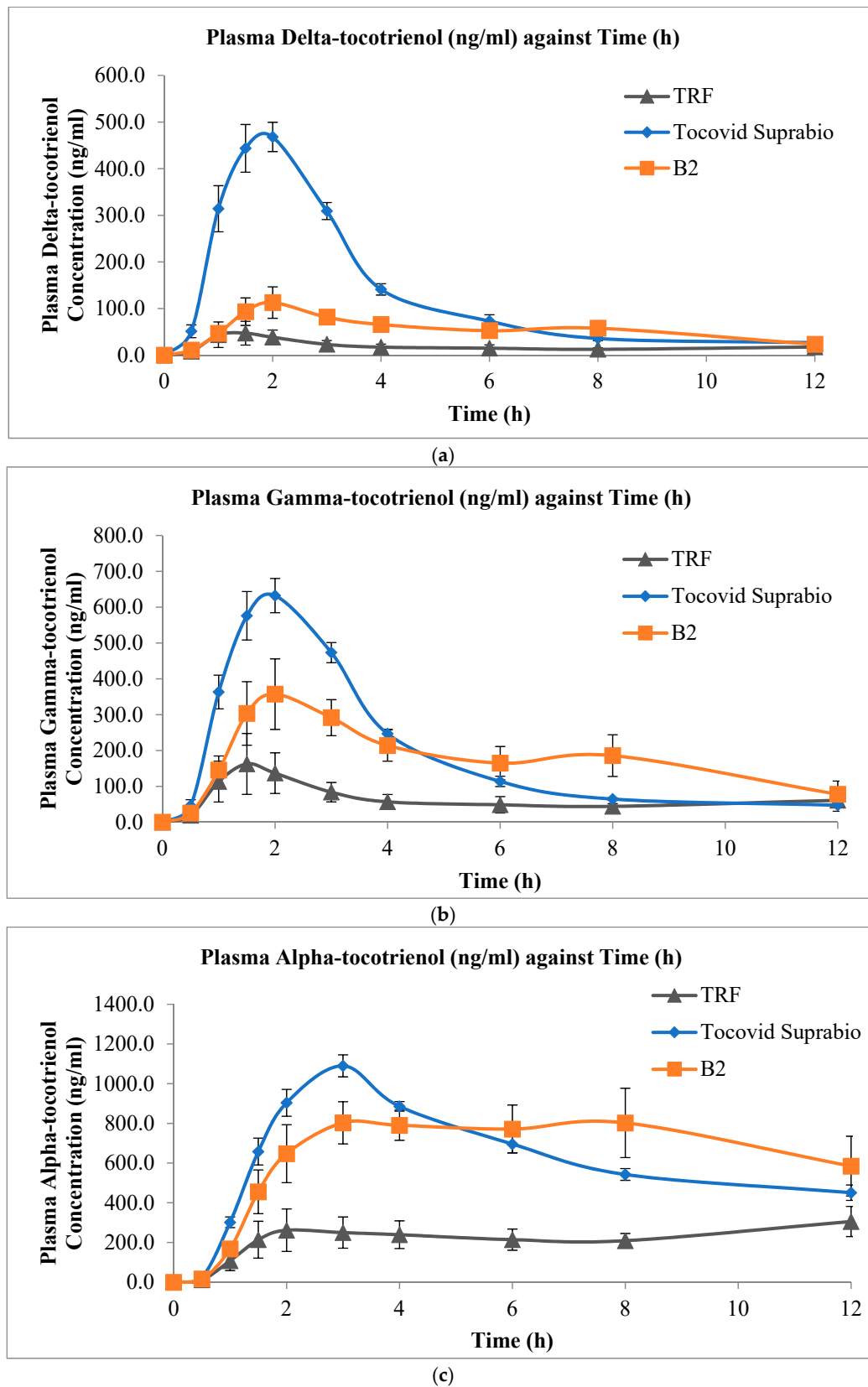
Figure 4. Mean plasma concentration versus time profiles (mean \pm SEM, n = 5 ) of (a) delta-tocotrienol; (b) gamma-tocotrienol; and (c) alpha-tocotrienol after oral administration of 20 mg/kg mixed tocotrienols in three different tocotrienol preparations: the non-self-emulsifying oily preparation (TRF), Tocovid Suprabio TM , and B2.
