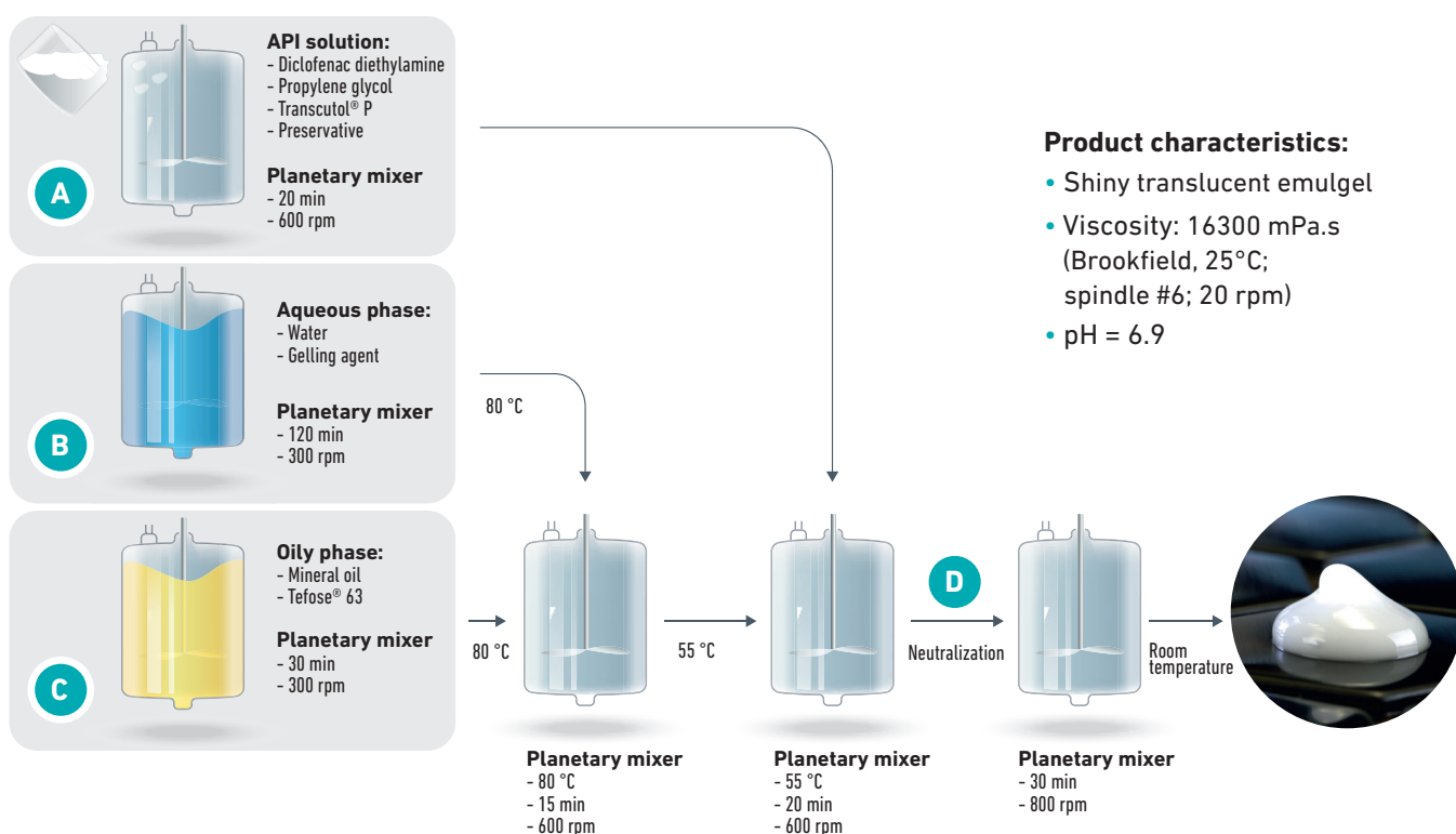
Figure 10: Emugel process (lab scale)
