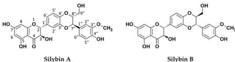
Figure 1: Molecular structures of Silybin A and B.
