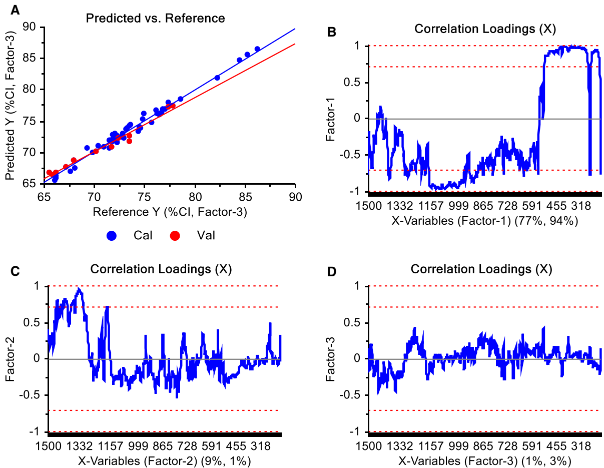
Fig. 7 a Values of crystallinity index (%CI) predicted by the Partial Least Square Regression model vs Reference values for the PhAT probe and considering three factors, and b, c, d correlation loadings of factors 1, 2, and 3, respectively, obtained from the model designed using baselined and
