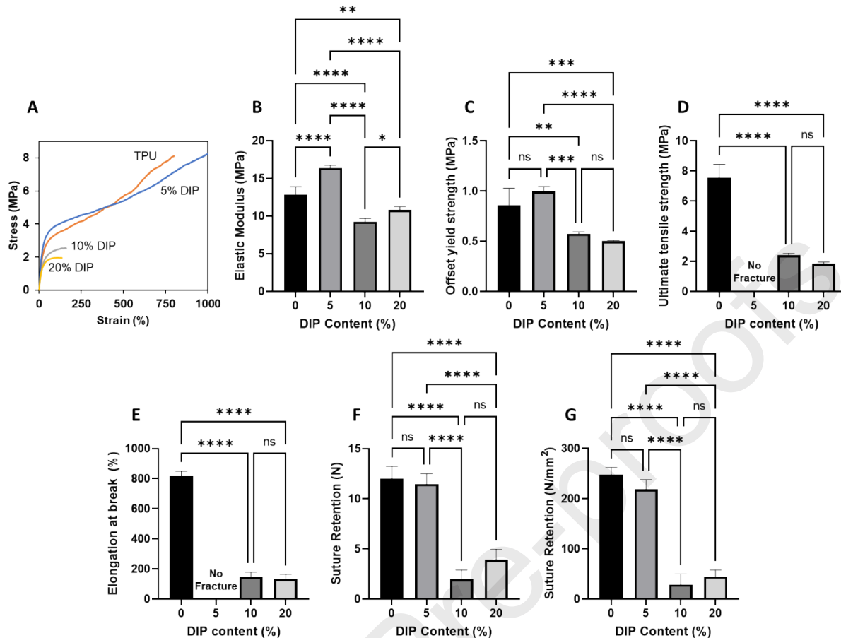
Figure 7. Representative stress/strain curves for the DIP-loaded 3D-printed samples (A). Elastic modulus (B), offset yield strength (C), ultimate tensile strength (D), elongation at break (E) and suture retention strength (F-G) for the DIP-loaded 3D-printed samples (n = 4).
