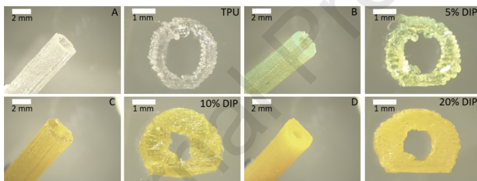
Figure 3. Light microscope images of the 3D-printed tubular grafts and their cross-sections. Scale bars are 1 and 2 mm.
