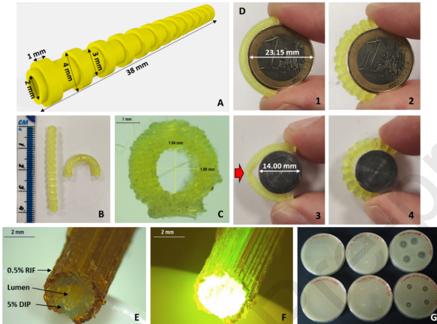
Figure 12. CAD design of anti-kinking vascular graft (A). Images of anti-kinking vascular graft and curved graft prepared using TPU containing 5% DIP (B). Light microscope image of the cross section of the anti-kinking vascular graft (C). Images showing plain grafts (1 and 3) and anti-kinking grafts (2 and 4) bent around cylindrical objects of different radius (D). Light microscope image of double-layer tubular graft (E) and the same image using the NIGHTSEA Model SFA Stereomicroscope Fluorescence Adapter (F). A picture showing the zones of inhibition obtained for S. aureus and E. coli in MH agar using slices of the double-layer tubular graft (G).
