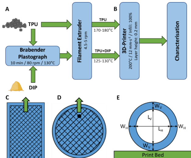
Figure 1. Diagram containing the different experimental phases, including mixing, hot-melt extrusion (A) and 3D-printing (B), used to prepare the 3D-printed small-diameter vascular grafts. Designs of the 3D printing strips (C) and discs (D) used to evaluate the uniaxial tensile mechanical properties and the suture retention strength test of the 3D-printed materials, respectively. The arrow indicates the tension direction during mechanical testing. Diagram showing the cross-section of a vascular graft and the different dimensions that were evaluated and presented in Table 1 (E).
