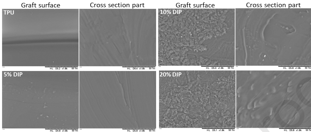
Figure 4. SEM images of the 3D-printed tubular grafts surfaces containing different DIP concentrations and their cross sections.
