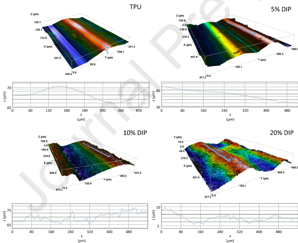
Figure 5. 3D images of the tubular grafts' surfaces containing different DIP concentrations and their topographic profiles studied in the direction of the predominant surface pattern determined by the 3D printing methodology.
