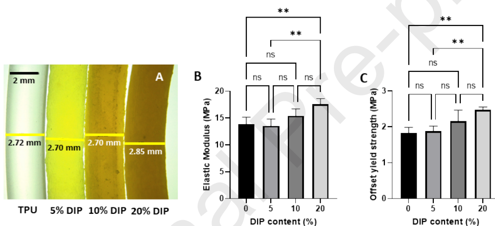
Figure 2. Light microscope image of the DIP-loaded TPU-based filaments (A). Elastic modulus (B) and offset yield strength (C) of the extruded filaments ( n = 4 ).
