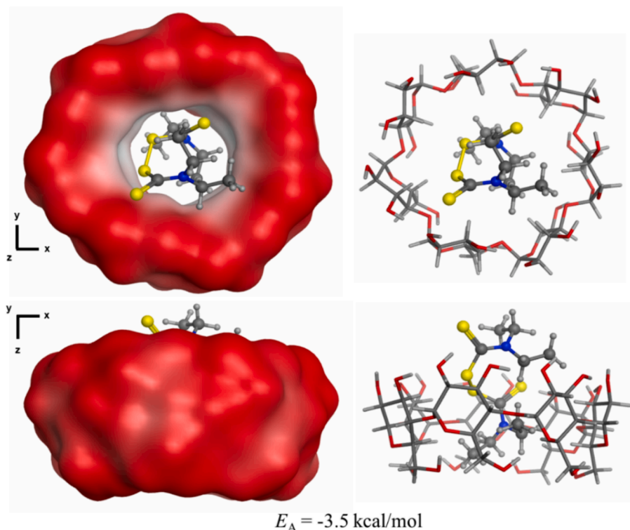
Fig. 2. Molecular modelling of spatial conformation of the DIS and \beta -CD inclusion complex and corresponding binding energy.
