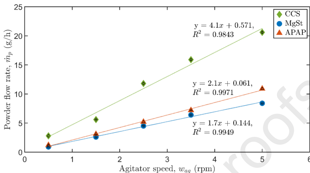
Figure 14: The summary of the powder flow rate as a function of agitator speed for the three different materials at optimal ratios, demonstrating a linear relationship. Experiments were conducted in triplicate ( n = 3 ).
