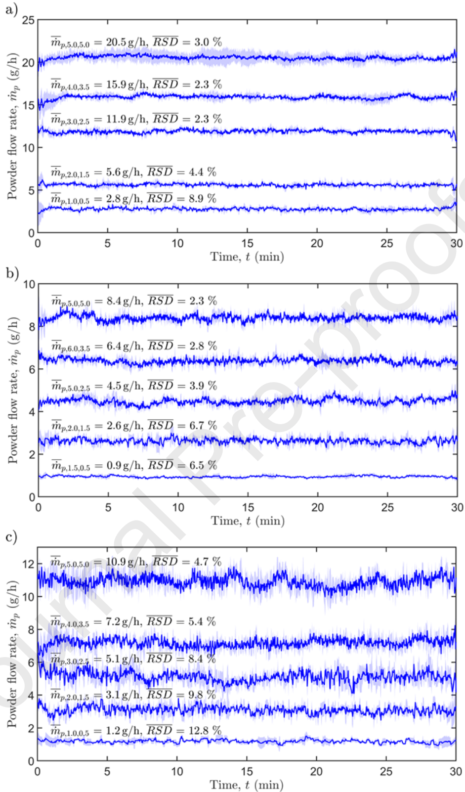
Figure 11: Consistent feeding of optimal ratios was observed in three repeat experiments without feedback control for (a) CCS, (b) MgSt, and (c) APAP. The blue line is the mean powder flow rate. The blue shadow represents the SD of three repeated experiments. A hopper refill at 20 minutes was performed.
