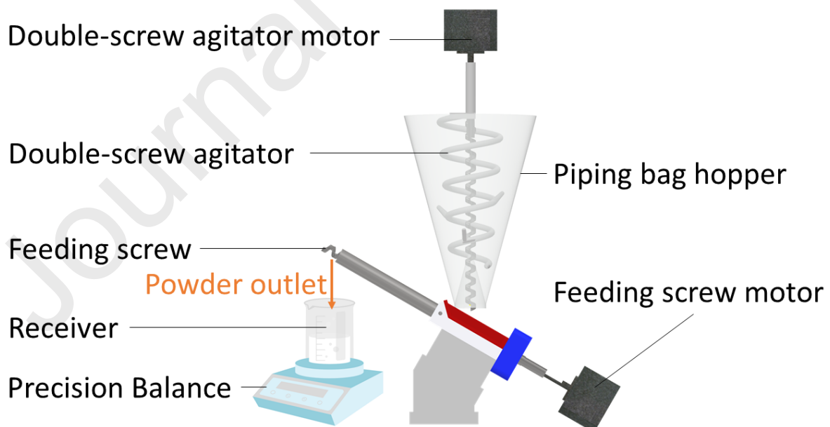
Figure 1: An overview of a schematic inclined micro-feeder.
