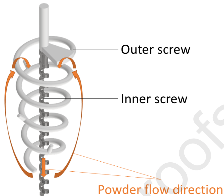
Figure 3: Schematic diagram of the double-screw agitator.
