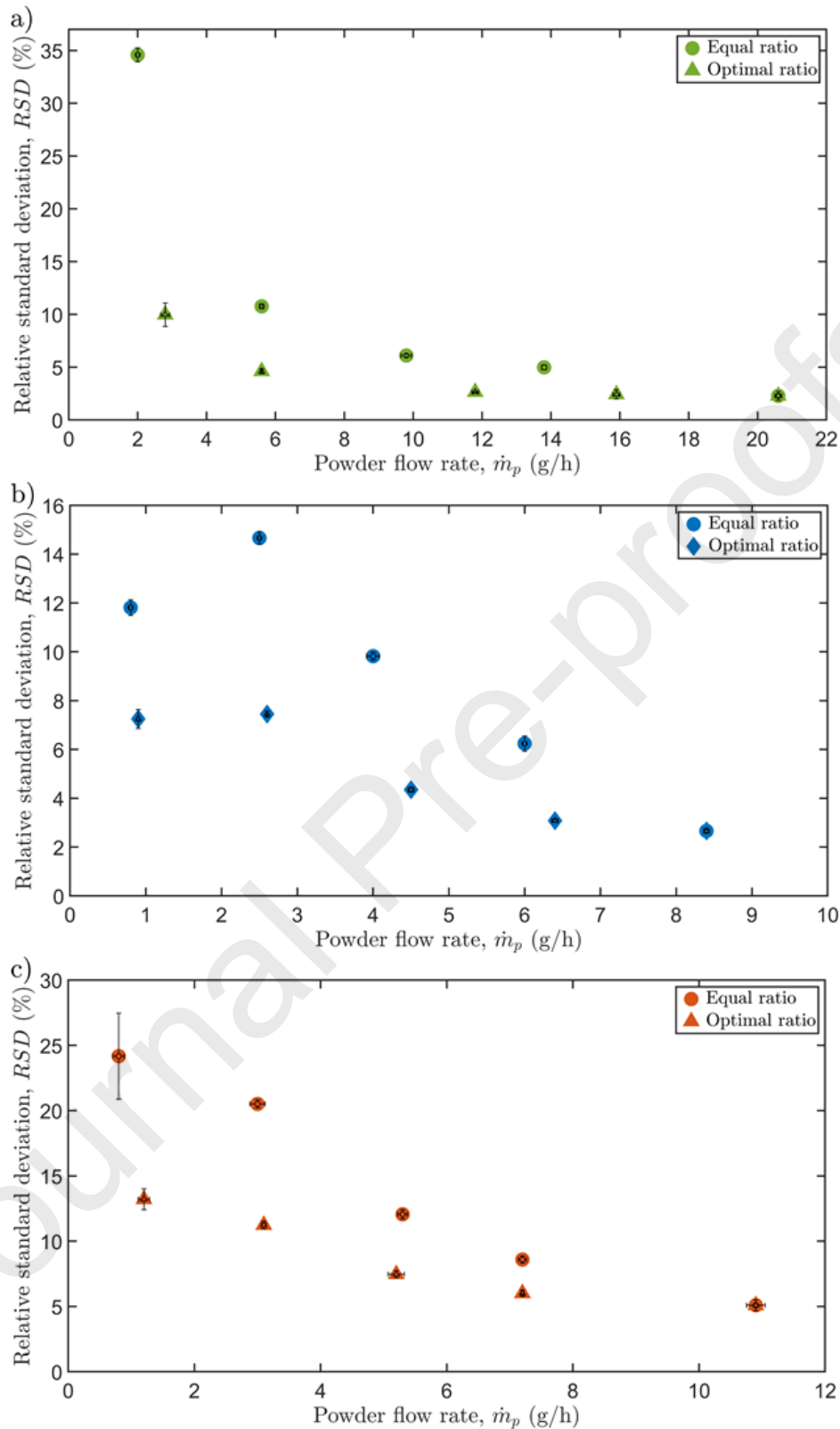
Figure 12: The summary statistics of the powder flow rates and RSDs for the three materials. RSDs as a function of powder flow rate at the equal and optimal ratio of screw and agitator speed a) CCS - Equal ratio: 20.6 g/h \pm 2.3% to 2.0 g/h \pm 34.6%; Optimal ratio: 20.6 g/h \pm 2.3% to 2.8 g/h \pm 10.0%; b) MgSt - Equal ratio: 8.4 g/h \pm 2.7% to 0.8 g/h \pm 11.8%; Optimal ratio: 8.4 g/h \pm 2.7% to 0.9 g/h \pm 7.3%; c) APAP - Equal ratio: 10.9 g/h \pm 5.1% to 0.8 g/h \pm 24.1%; Optimal ratio: 10.9 \pm 5.0% to 1.2 g/h \pm 13.2%. Horizontal and
