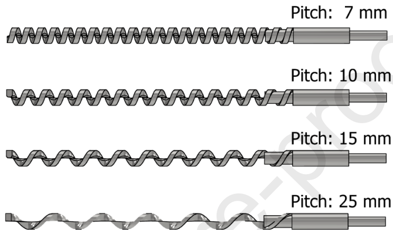
Figure 2: Schematic diagram of the feeding screws in four pitches: 7 mm, 10 mm, 15 mm and 25 mm.
