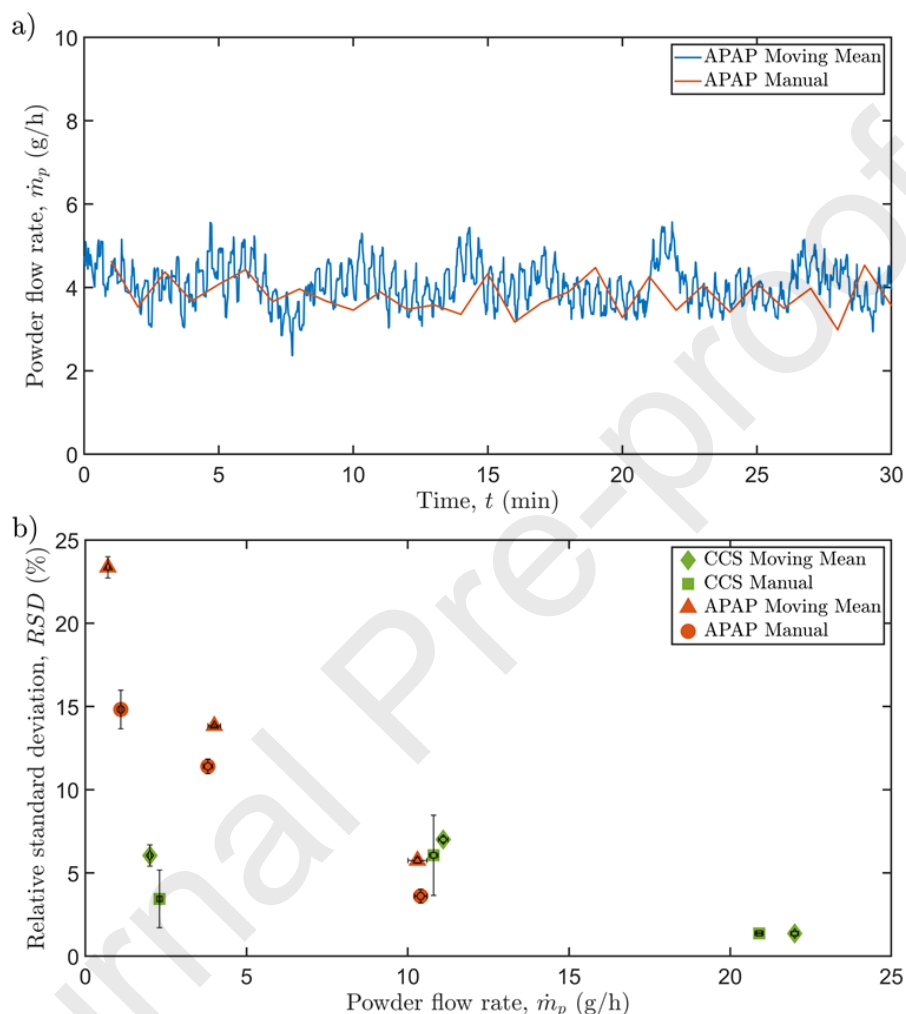
Figure 5: Effect of powder flow rate on RSD for automated and manual operation with 60-second window measurement, and APAP with lowest powder rate at 120-second window measurement. a) an illustration of APAP feeding conducted over a 30-minute duration, with manual measurements recorded at one-minute intervals, juxtaposed with automatic data acquisition utilising a 1-minute moving mean filter; b) a comprehensive summary of the results obtained from both manual and automatic measurements. Each measurement was done in triplicate ( n = 3 ). The vertical error bar represents the standard deviation of relative standard deviations of three repeat experiments. The horizontal error bar represents the standard deviation of powder flow rates of three repeat experiments. The statistical comparison of data set can be found in Table S1 in the Supporting Information.
