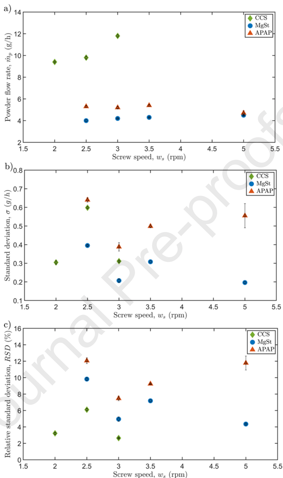
Figure 10: Effects of feeding screw speed on powder flow rate, SD and RSD for three distinct powder properties. a) Mean powder flow rate of three repeat experiments ( n = 3 ) as a function of feeding screw speed for three different powder properties at a constant double-screw agitator speed of 2.5 rpm; b) standard deviation as a function of feeding screw speed at 2.5 rpm of double-screw agitator speed; c) relative standard deviation as a function of feeding screw speed at 2.5 rpm of double-screw agitator speed.
