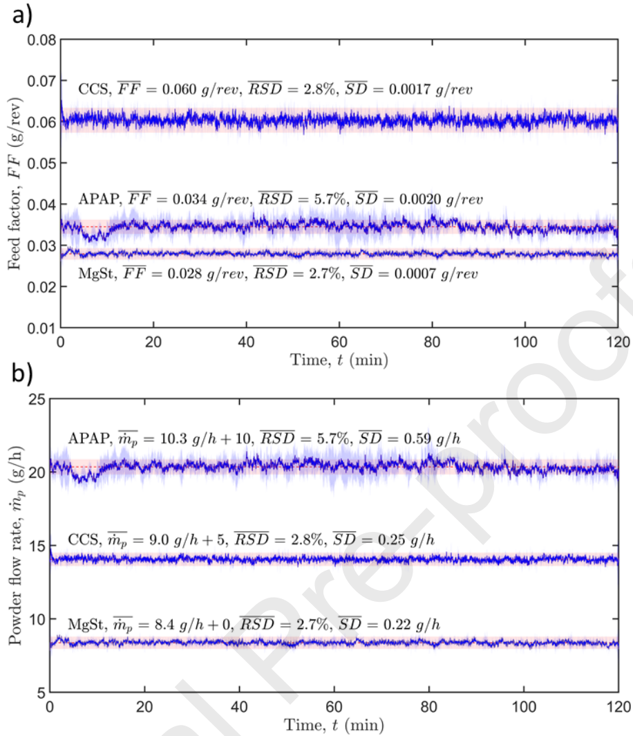
Figure 6: Refilling every 20 min in continuous feeding demonstrated for three different materials: a) Feed factor over time, b) Changes in powder flow rate with respect to feeding time. All experiments were performed in triplicates ( n = 3 ). The blue line is the mean powder flow rate. The blue shadow represents the SD of three repeated experiments. The red shaded belt represents \pm 5\% . The notation "XX g/h+Number" is used to shift the trend up by "Number" g/h for comparison purposes.
