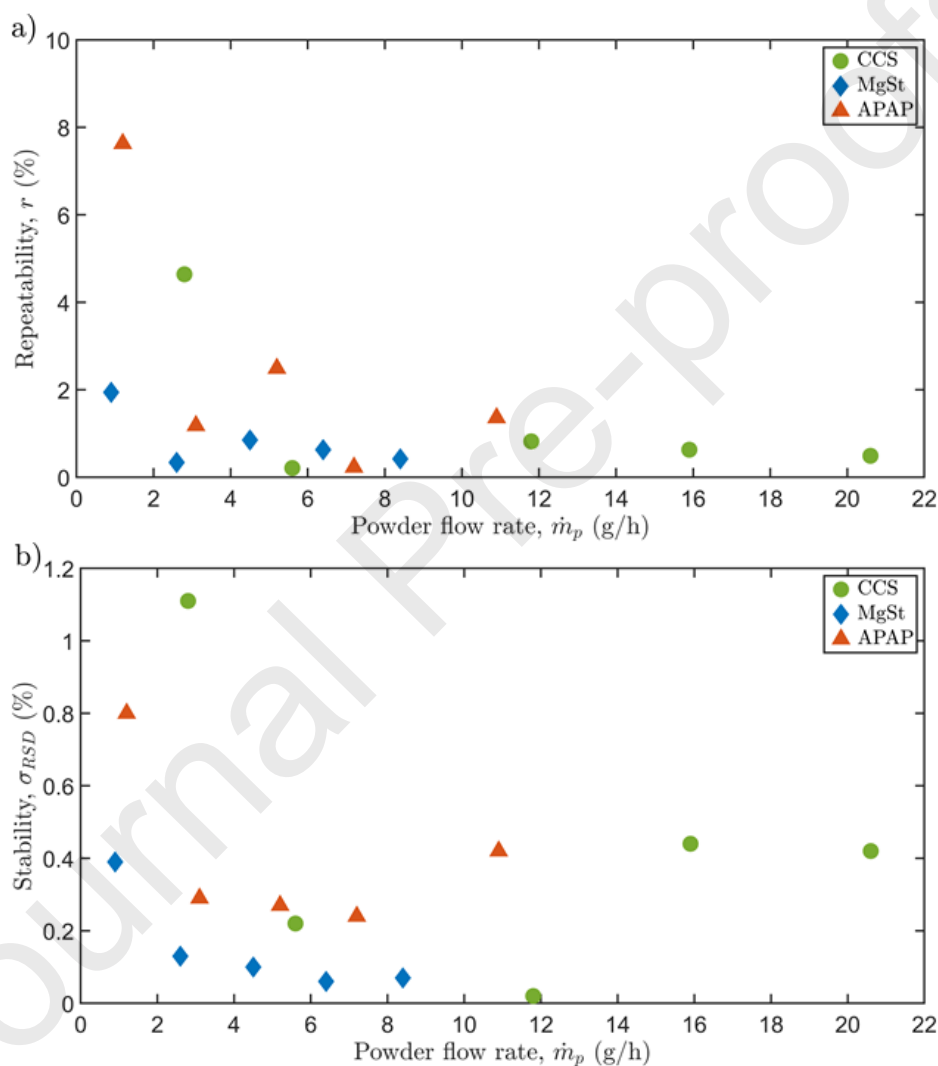
Figure 13: Repeatability and stability at the optimal ratios were investigated for the three materials. a) repeatability and b) stability as a function of powder flow rate at the optimal ratio. The agitator speed was kept constant rather than the feed rate. Due to the differing physical properties of the three investigated powders, the average feed rate varies at a constant agitator speed.
