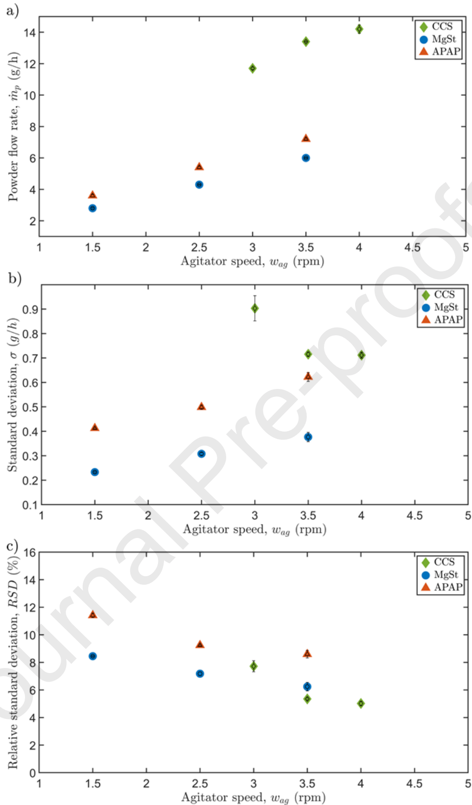
Figure 8: The effect of double-screw agitator speed on powder flow rate, SD and RSD. a) The mean powder flow rate from three repeated experiments ( n = 3 ) is plotted against agitator speed for three different powder properties at a fixed feeding screw speed of 3.5 rpm. b) SD is plotted against agitator speed. c) RSD is plotted against agitator speed.
