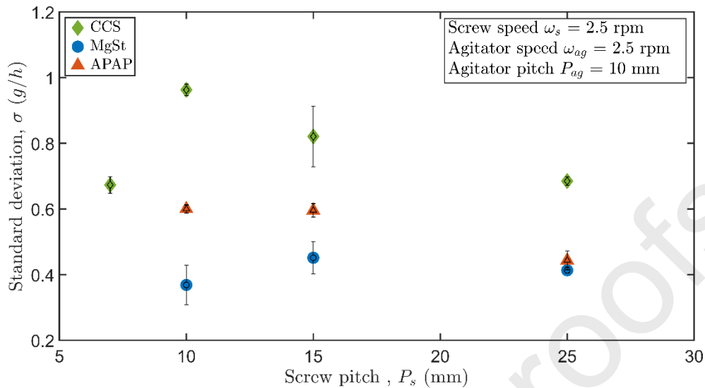
Figure 7: Standard deviation as a function of screw pitches for CCS, MgSt and APAP. Each measurement was done in triplicate ( n = 3 ).
