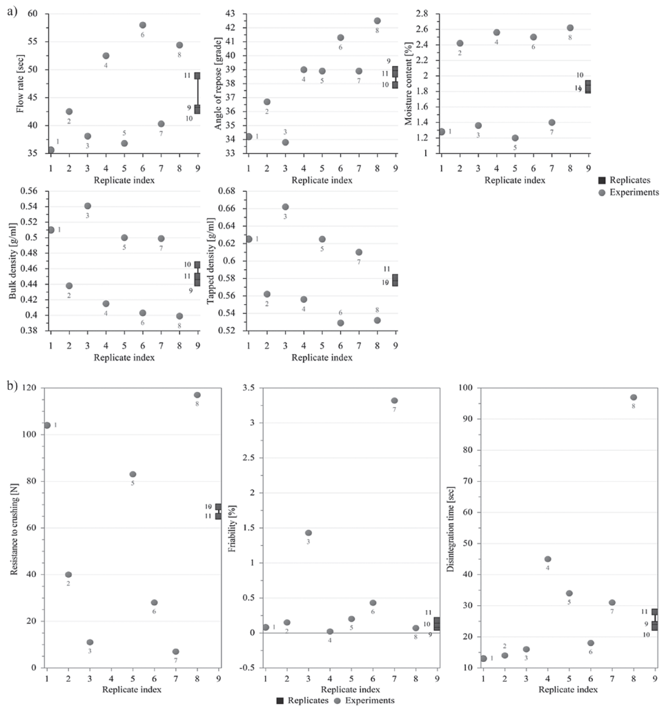
Fig. 1. Replicate plot of responses: a) model for powder properties, b) model for tablet properties. Numbers represent individual experiments.
