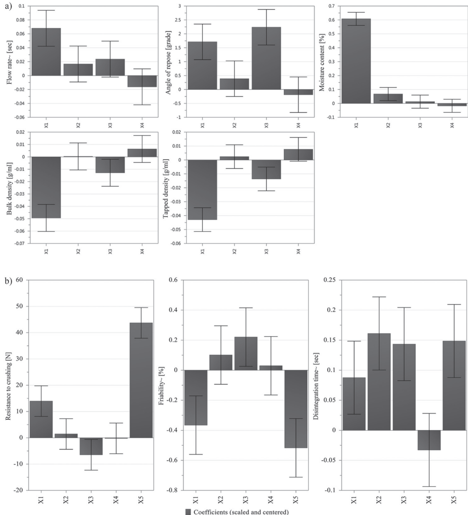
Fig. 3. Coefficient plots for responses: a) model for powder properties, b) model for tablet properties. X1 – MCC proportion (%), X2 – sodium croscarmellose proportion (%), X3 – MgSt proportion (%), X4 – bending time with lubricant (min), X5 – compression force (kN).
